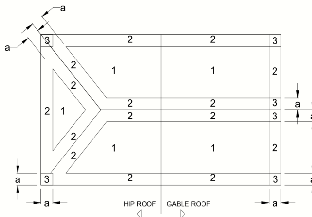
a: 10% OF LEAST HORIZONTAL DIMENSION OR 0.4h, WHICHEVER IS SMALLER, BUT NOT LESS THAN EITHER 4% OF LEAST HORIZONTAL DIMENSION OR 3FT (0.9M), OR AS DETERMINED BY DESIGN OR OTHER APPLICABLE CODE.
